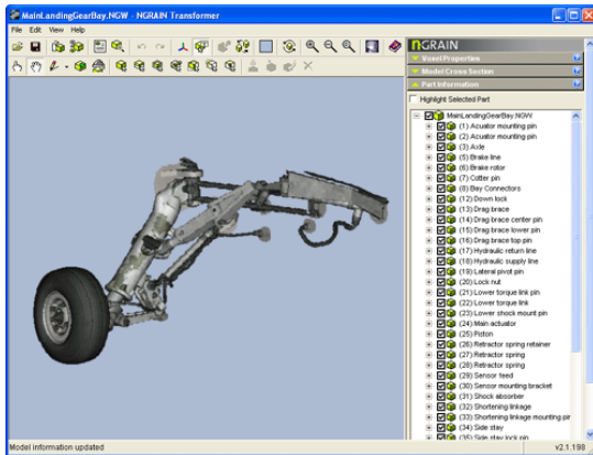
Figure 10. 3D Landing Gear model converted using NGRAIN® Transformer
